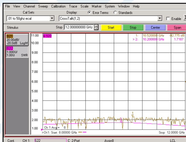
(J1 – J3) Insertion Loss and Return Loss
