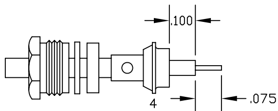
ASSEMBLY (B)
