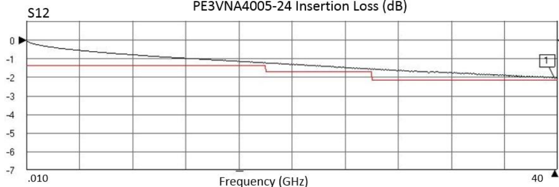
PE3VNA4005-24 Insertion Loss (dB)
