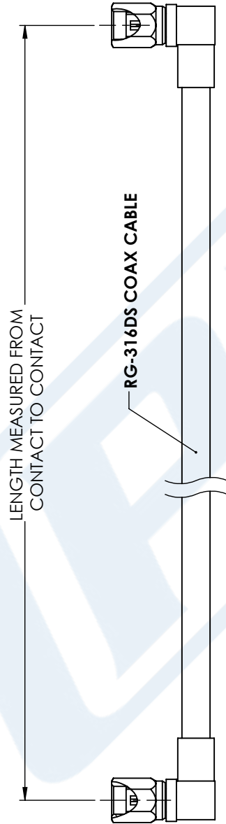
2X, SSMC PLUG RIGHT ANGLE CONNECTOR
