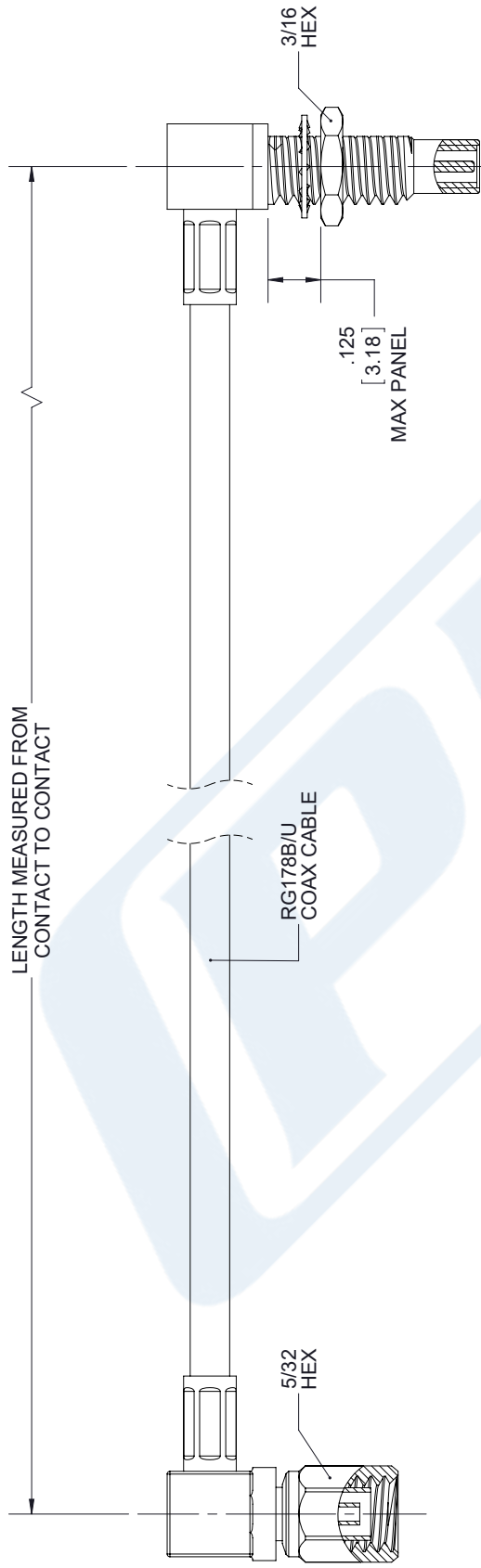
SSMC R.A JACK BULKHEAD MOUNT CONNECTOR
