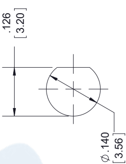
MOUNTING HOLE
