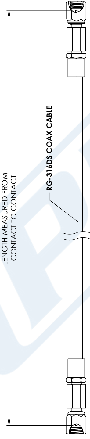
2X, SSMC PLUG CONNECTOR
